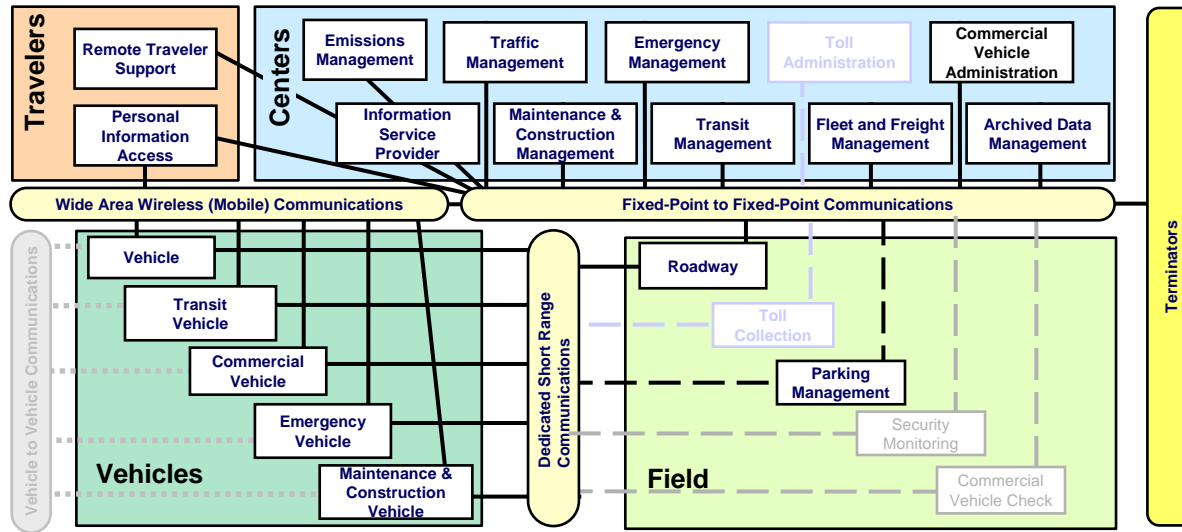
Lufkin Region, Texas Regional ITS Architecture "Sausage Diagram"
