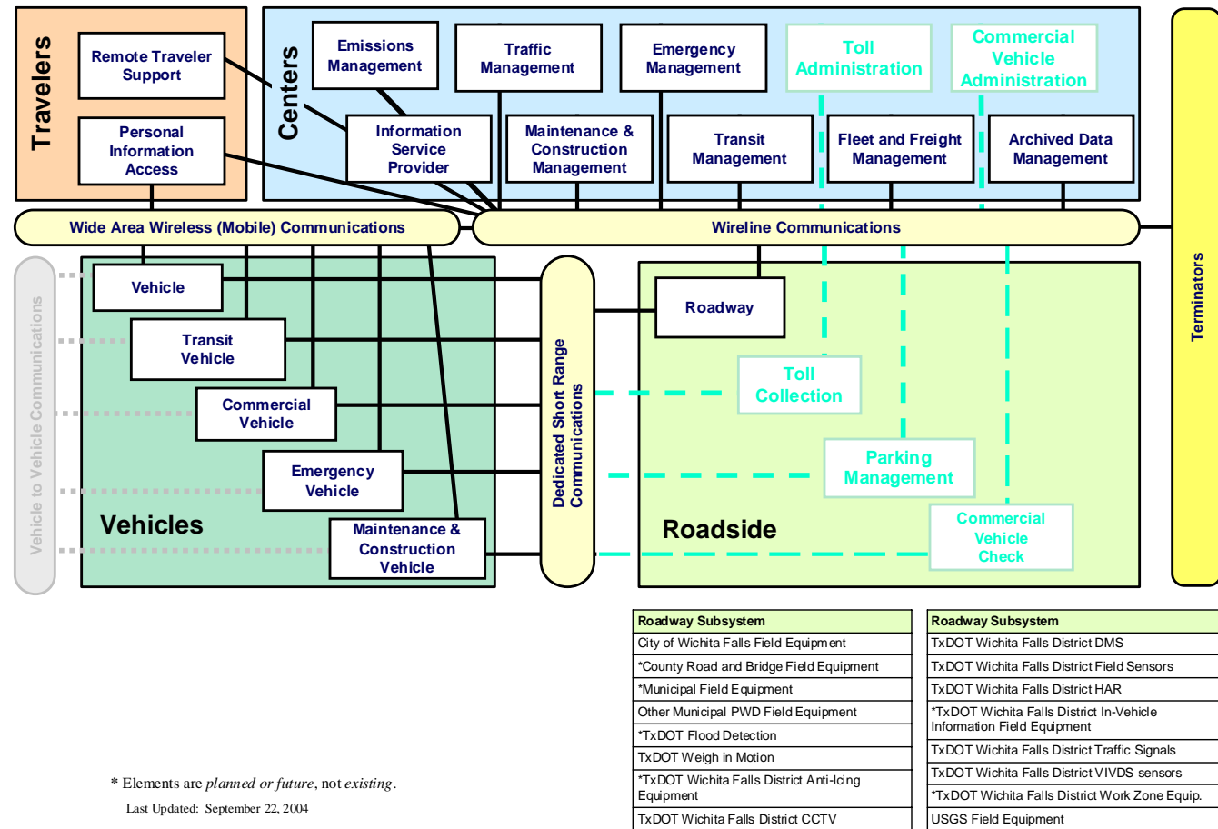
Figure 5 – Wichita Falls Regional System Interconnect Diagram
